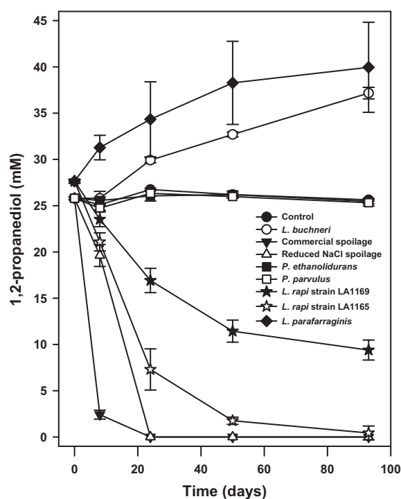
Fig. 4. Utilization of 1,2-propanediol in fermented cucumber medium (6% NaCl, pH 3.8) by spoilage cultures and Lactobacillus rari . Control samples were not inoculated.
