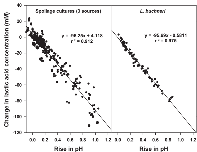
Fig. 3. Rise in pH correlated with anaerobic D/L-lactic acid utilization in fermented cucumber media (initial pH 3.1–3.8) regardless of NaCl concentration (0–6%) by spoilage cultures from three sources ( n = 366 ) and L. buchneri ( n = 77 ).
